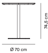
Form Café Table Linoleum
