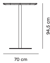
Form Café Table Linoleum
